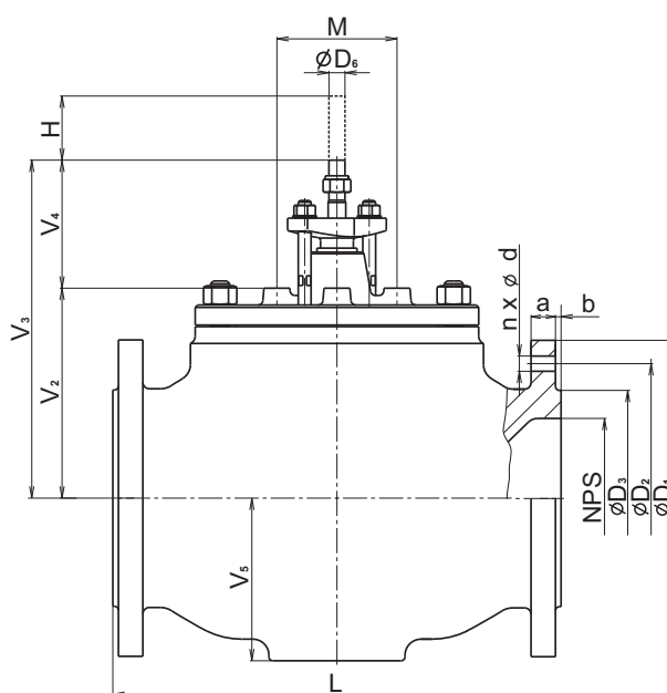
NPS 8" - 10"
