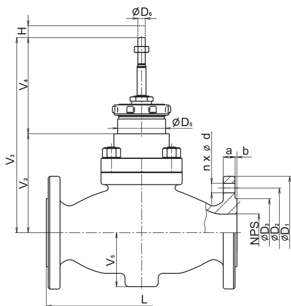
NPS 1" - 6"
