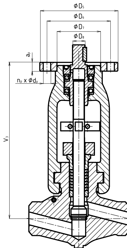
Valve ready for actuator connection (EXX execution)
